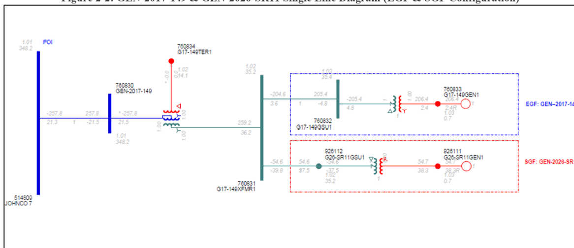
Figure 2-2: GEN-2017-149 & GEN-2026-SR11 Single Line Diagram (EGF & SGF Configuration)
