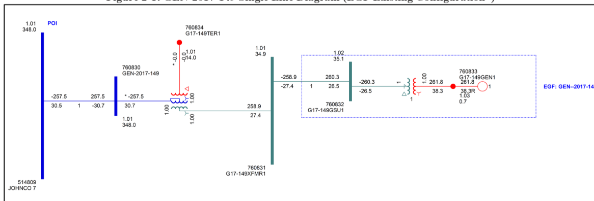
Figure 2-1: GEN-2017-149 Single Line Diagram (EGF Existing Configuration*)
